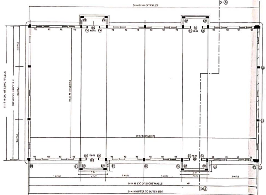
PLAN FOR PROCESSING UNIT UNIT NO 1. II
