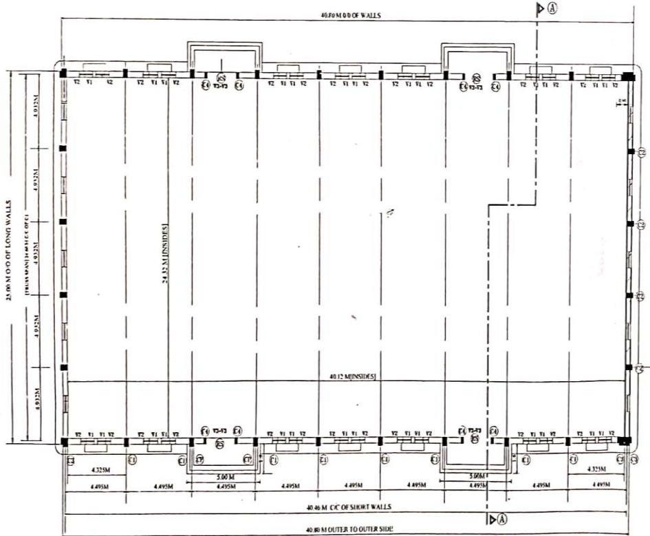
PLAN FOR 1800 MT. WAREHOUSE UNIT NO. 1.II
